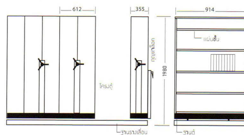
CPT 6, 8, 10 (Side View)
