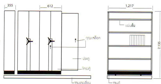
CPT 5, 7, 9 (Side View)
